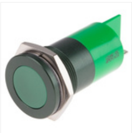
RS PRO Green Indicator, 12 V, 22mm Mounting Hole Size, Faston, Solder Lug Termination, IP67, Индикатор Stock number: 8987712
