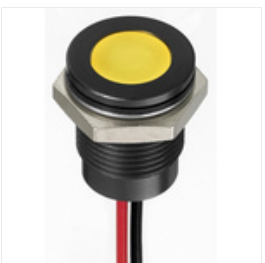
RS PRO Yellow Indicator, 24 V dc, 14mm Mounting Hole Size, Lead Wires Termination, IP67, Индикатор Stock number: 1302299
