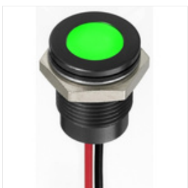
RS PRO Green Indicator, 1.8 → 3.3 V dc, 14mm Mounting Hole Size, Lead Wires Termination, IP67, Индикатор Stock number: 1302288
