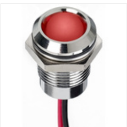
RS PRO Red Indicator, 220 V ac, 14mm Mounting Hole Size, Lead Wires Termination, IP67, Индикатор Stock number: 1301092
