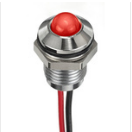
RS PRO Red Indicator, 12 V dc, 8mm Mounting Hole Size, Lead Wires Termination, IP67, Индикатор Stock number: 1329103
