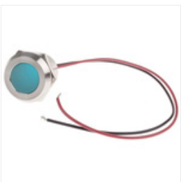
RS PRO Blue Indicator, 12 V dc, 22mm Mounting Hole Size, Lead Wires Termination, IP67, Индикатор Stock number: 1232435
