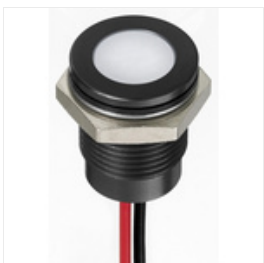
RS PRO White Indicator, 1.8 → 3.3 V dc, 14mm Mounting Hole Size, Lead Wires Termination, IP67, Индикатор Stock number: 1302291
