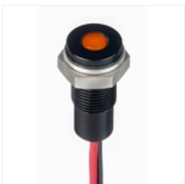
RS PRO Orange Panel LED, 10.8 → 13.2 V dc, 6mm Mounting Hole Size, Lead Wires Termination, IP67, Индикатор Stock number: 1713827
