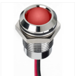
RS PRO Red Indicator, 1.8 → 3.3 V dc, 14mm Mounting Hole Size, Lead Wires Termination, IP67, Индикатор Stock number: 1301074
