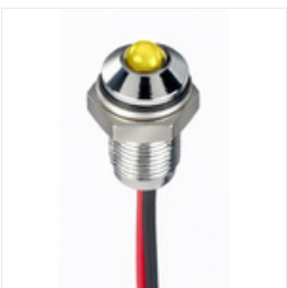
RS PRO Yellow Panel LED, 21.6 → 26.4 V dc, 6mm Mounting Hole Size, Lead Wires Termination, IP67, Индикатор Stock number: 1713765
