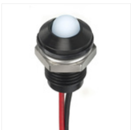
RS PRO White Indicator, 1.8 → 3.3 V dc, 8mm Mounting Hole Size, Lead Wires Termination, IP67, Индикатор Stock number: 1329132
