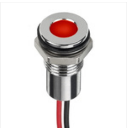
RS PRO Red Indicator, 24 V dc, 8mm Mounting Hole Size, Lead Wires Termination, IP67, Индикатор Stock number: 1329123
