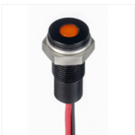
RS PRO Orange Panel LED, 21.6 → 26.4 V dc, 6mm Mounting Hole Size, Lead Wires Termination, IP67, Индикатор Stock number: 1713834
