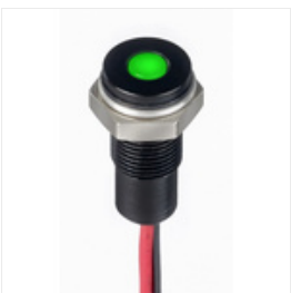
RS PRO Green Panel LED, 1.8 → 3.3 V dc, 6mm Mounting Hole Size, Lead Wires Termination, IP67, Индикатор Stock number: 1713816
