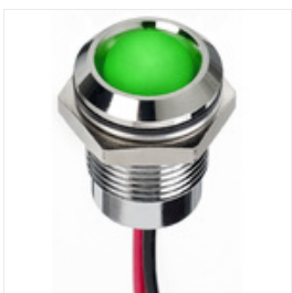
RS PRO Green Indicator, 24 V dc, 14mm Mounting Hole Size, Lead Wires Termination, IP67, Индикатор Stock number: 1301085
