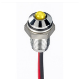
RS PRO Yellow Panel LED, 10.8 → 13.2 V dc, 6mm Mounting Hole Size, Lead Wires Termination, IP67, Индикатор Stock number: 1713758
