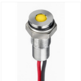
RS PRO Yellow Panel LED, 10.8 → 13.2 V dc, 6mm Mounting Hole Size, Lead Wires Termination, IP67, Индикатор Stock number: 1713780
