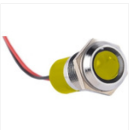
RS PRO Yellow Indicator, 220 V ac, 14mm Mounting Hole Size, Lead Wires Termination, IP67, Индикатор Stock number: 7227485
