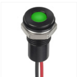
RS PRO Green Indicator, 1.8 → 3.3 V dc, 8mm Mounting Hole Size, Lead Wires Termination, IP67, Индикатор Stock number: 1329144
