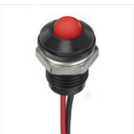
RS PRO Red Indicator, 1.8 → 3.3 V dc, 8mm Mounting Hole Size, Lead Wires Termination, IP67, Индикатор Stock number: 1329128
