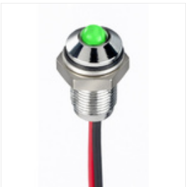
RS PRO Green Panel LED, 1.8 → 3.3 V dc, 6mm Mounting Hole Size, Lead Wires Termination, IP67, Индикатор Stock number: 1713749
