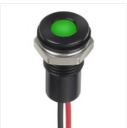
RS PRO Green Indicator, 12 V dc, 8mm Mounting Hole Size, Lead Wires Termination, IP67, Индикатор Stock number: 1329149
