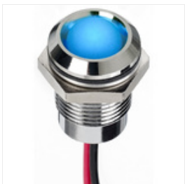
RS PRO Blue Indicator, 1.8 → 3.3 V dc, 14mm Mounting Hole Size, Lead Wires Termination, IP67, Индикатор Stock number: 1301077
