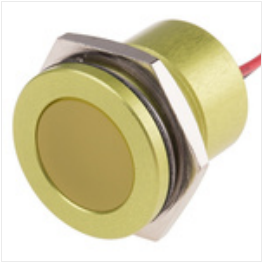
RS PRO Yellow Indicator, 24 V ac/dc, 22mm Mounting Hole Size, Lead Wires Termination, IP67, Индикатор Stock number: 8987766
