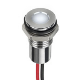
RS PRO White Indicator, 1.8 → 3.3 V dc, 8mm Mounting Hole Size, Lead Wires Termination, IP67, Индикатор Stock number: 1329117
