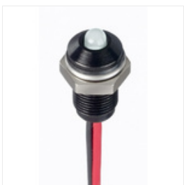
RS PRO White Panel LED, 10.8 → 13.2 V dc, 6mm Mounting Hole Size, Lead Wires Termination, IP67, Индикатор Stock number: 1713804
