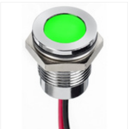
RS PRO Green Indicator, 12 V dc, 14mm Mounting Hole Size, Lead Wires Termination, IP67, Индикатор Stock number: 1301101
