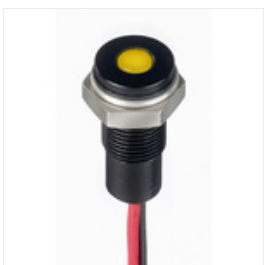
RS PRO Yellow Panel LED, 10.8 → 13.2 V dc, 6mm Mounting Hole Size, Lead Wires Termination, IP67, Индикатор Stock number: 1713824
