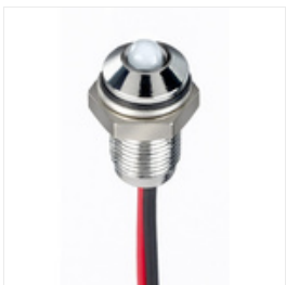
RS PRO White Panel LED, 10.8 → 13.2 V dc, 6mm Mounting Hole Size, Lead Wires Termination, IP67, Индикатор Stock number: 1713760
