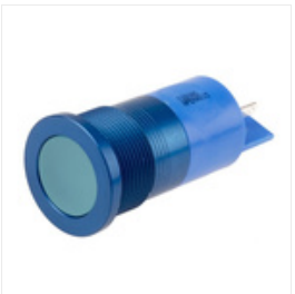
RS PRO Blue Indicator, 110 V ac, 22mm Mounting Hole Size, Faston, Solder Lug Termination, IP67, Индикатор Stock number: 8987797
