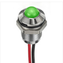
RS PRO Green Indicator, 12 V dc, 8mm Mounting Hole Size, Lead Wires Termination, IP67, Индикатор Stock number: 1329104
