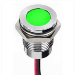
RS PRO Green Indicator, 1.8 → 3.3 V dc, 14mm Mounting Hole Size, Lead Wires Termination, IP67, Индикатор Stock number: 1301096
