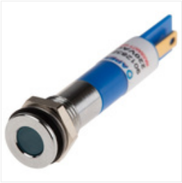
RS PRO Blue Indicator, 220 V ac, 8mm Mounting Hole Size, Solder Lug Termination, IP67, Индикатор Stock number: 8462917
