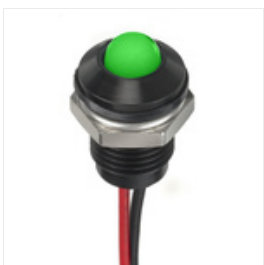
RS PRO Green Indicator, 24 V dc, 8mm Mounting Hole Size, Lead Wires Termination, IP67, Индикатор Stock number: 1329139
