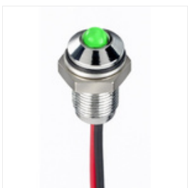
RS PRO Green Panel LED, 21.6 → 26.4 V dc, 6mm Mounting Hole Size, Lead Wires Termination, IP67, Индикатор Stock number: 1713764
