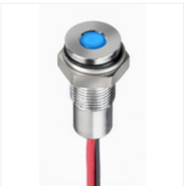
RS PRO Blue Panel LED, 1.8 → 3.3 V dc, 6mm Mounting Hole Size, Lead Wires Termination, IP67, Индикатор Stock number: 1713773
