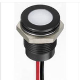
RS PRO White Indicator, 12 V dc, 14mm Mounting Hole Size, Lead Wires Termination, IP67, Индикатор Stock number: 1302296
