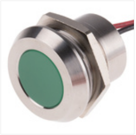
RS PRO Green Indicator, 28 V dc, 22mm Mounting Hole Size, Lead Wires Termination, IP67, Индикатор Stock number: 1232429
