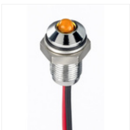
RS PRO Orange Panel LED, 21.6 → 26.4 V dc, 6mm Mounting Hole Size, Lead Wires Termination, IP67, Индикатор Stock number: 1713768
