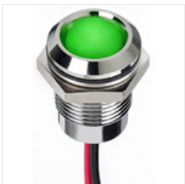
RS PRO Green Indicator, 1.8 → 3.3 V dc, 14mm Mounting Hole Size, Lead Wires Termination, IP67, Индикатор Stock number: 1301075
