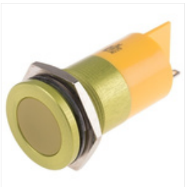
RS PRO Yellow Indicator, 110 V ac, 22mm Mounting Hole Size, Faston, Solder Lug Termination, IP67, Индикатор Stock number: 8987750
