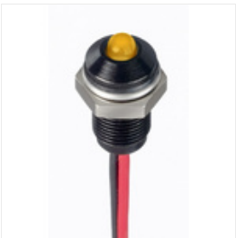
RS PRO Yellow Panel LED, 21.6 → 26.4 V dc, 6mm Mounting Hole Size, Lead Wires Termination, IP67, Индикатор Stock number: 1713810
