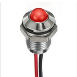
RS PRO Red Indicator, 24 V dc, 8mm Mounting Hole Size, Lead Wires Termination, IP67, Индикатор Stock number: 1329108
