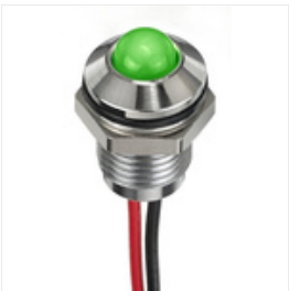
RS PRO Green Indicator, 24 V dc, 8mm Mounting Hole Size, Lead Wires Termination, IP67, Индикатор Stock number: 1329109
