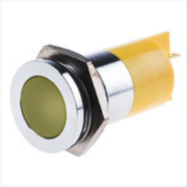
RS PRO Yellow Indicator, 110 V dc, 22mm Mounting Hole Size, Solder Lug Termination, IP67, Индикатор Stock number: 8332917
