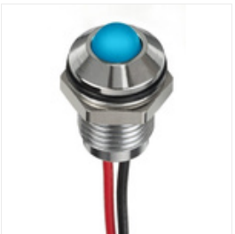
RS PRO Blue Indicator, 24 V dc, 8mm Mounting Hole Size, Lead Wires Termination, IP67, Индикатор Stock number: 1329111
