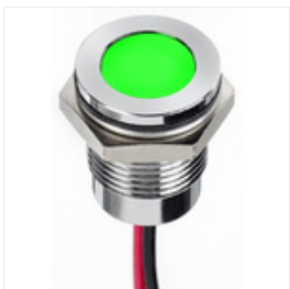
RS PRO Green Indicator, 24 V dc, 14mm Mounting Hole Size, Lead Wires Termination, IP67, Индикатор Stock number: 1302260
