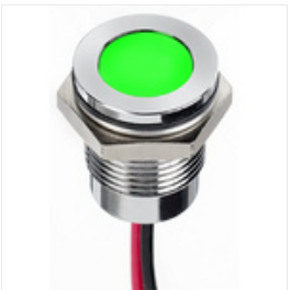
RS PRO Green Indicator, 220 V ac, 14mm Mounting Hole Size, Lead Wires Termination, IP67, Индикатор Stock number: 1302267
