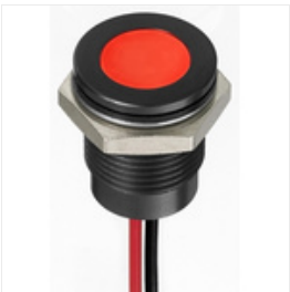
RS PRO Red Indicator, 1.8 → 3.3 V dc, 14mm Mounting Hole Size, Lead Wires Termination, IP67, Индикатор Stock number: 1302287
