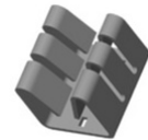
RS PRO Heatsink, 11 (Forced) °C/W, 29 (Natural) °C/W, 15.2 x 13.6 x 12.7mm, Bolt On, Horizontal, Vertical, Радиатор
