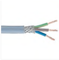
RS PRO 3 Core CY Control Cable 0.75 mm 2 , 50m, Screened, Кабель Stock number: 0522519
