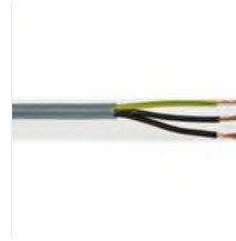
RS PRO 8 Core YY Control Cable, 1.5 mm 2 , 50m, Unscreened, Кабель
