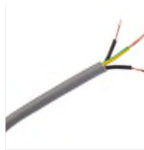
RS PRO 3 Core YY Control Cable, 1 mm 2 , 50m, Unscreened
