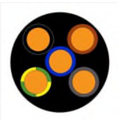
RS PRO 5 Core 1.5 mm 2 Mains Power Cable, Polyvinyl Chloride PVC Sheath 100m, 20 A 300/500 V, TUF Stock number: 6755668
