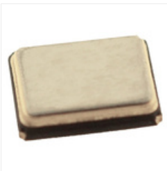
RS PRO 16MHz Crystal \pm 20 ppm SMT 4-Pin 3.2 x 2.5 x 0.7mm
