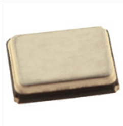
RS PRO 27MHz Crystal \pm 10 ppm SMT 4-Pin 3.2 x 2.5 x 0.7mm Stock number: 1445086
