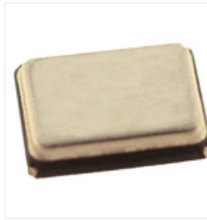
RS PRO 16MHz Crystal \pm 50 ppm SMT 4-Pin 3.2 x 2.5 x 0.7mm
