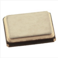
RS PRO 12MHz Crystal \pm 20 ppm SMT 4-Pin 3.2 x 2.5 x 0.7mm Stock number: 1445052
