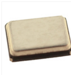
RS PRO 12MHz Crystal \pm 10\text{ppm} SMT 4-Pin 3.2 x 2.5 x 0.7mm
