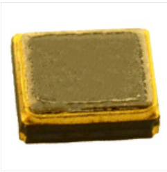
RS PRO 26MHz TCXO Oscillator, Clipped Sinewave \pm 1.5\text{ppm} SMD
