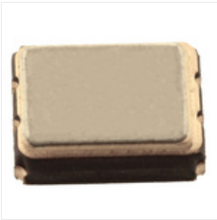
RS PRO 26MHz TCXO Oscillator, CMOS SMD
