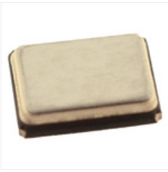
RS PRO 25MHz Crystal \pm 10 ppm SMT 4-Pin 3.2 x 2.5 x 0.7mm
