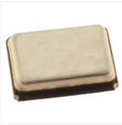
RS PRO 48MHz Crystal \pm 10 ppm SMT 4-Pin 3.2 x 2.5 x 0.7mm
