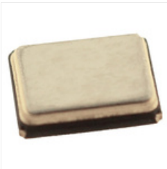
RS PRO 18.432MHz Crystal \pm 30 ppm SMT 4-Pin 3.2 x 2.5 x 0.7mm
