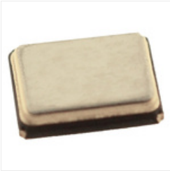
RS PRO 25MHz Crystal \pm 30 ppm SMT 4-Pin 3.2 x 2.5 x 0.7mm
