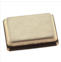
RS PRO 12MHz Crystal \pm 30 ppm SMT 4-Pin 3.2 x 2.5 x 0.7mm
