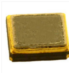
RS PRO 40MHz TCXO Oscillator, Clipped Sinewave \pm 1.5\text{ppm} SMD
