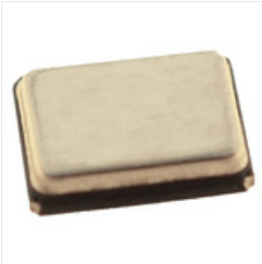
RS PRO 27.12MHz Crystal \pm 30 ppm SMT 4-Pin 3.2 x 2.5 x 0.7mm Stock number: 1445088
