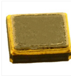
RS PRO 32MHz TCXO Oscillator, Clipped Sinewave \pm 1.5\text{ppm} SMD
