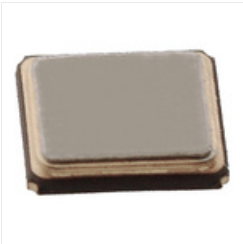
RS PRO 12MHz Crystal \pm 30 ppm SMT 4-Pin 2.5 x 2 x 0.5mm
