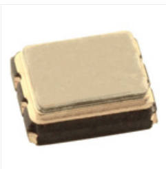
RS PRO, 25MHz Clock Oscillator, \pm 50\text{ppm} HCMOS, 4-Pin SMD, Тактовый генератор Stock number: 1445009
