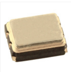
RS PRO, 25MHz Clock Oscillator, \pm 50\text{ppm} HCMOS, 4-Pin SMD, Тактовый генератор Stock number: 1445010
