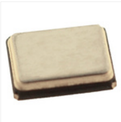
RS PRO 50MHz Crystal \pm 10\text{ppm} SMT 4-Pin 3.2 x 2.5 x 0.7mm
