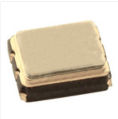
RS PRO, 4MHz Clock Oscillator, \pm 50\text{ppm} HCMOS, 4-Pin SMD, Тактовый генератор Stock number: 1445011
