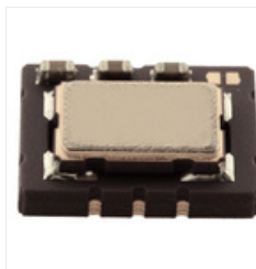
RS PRO 24.57MHz TCXO Oscillator, HCMOS, TTL \pm 0.028\text{ppm} SMD Stock number: 1442373
