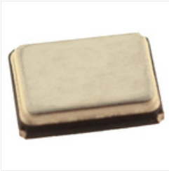
RS PRO 16MHz Crystal \pm 10 ppm SMT 4-Pin 3.2 x 2.5 x 0.7mm
