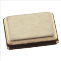
RS PRO 25MHz Crystal \pm 20 ppm SMT 4-Pin 3.2 x 2.5 x 0.7mm
