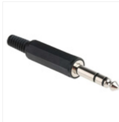
RS PRO 6.35 mm Cable Mount Stereo Jack Plug, 3Pole Stock number: 0392665
