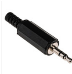
RS PRO 3.5 mm Cable Mount Stereo Jack Plug Stock number: 0392643
